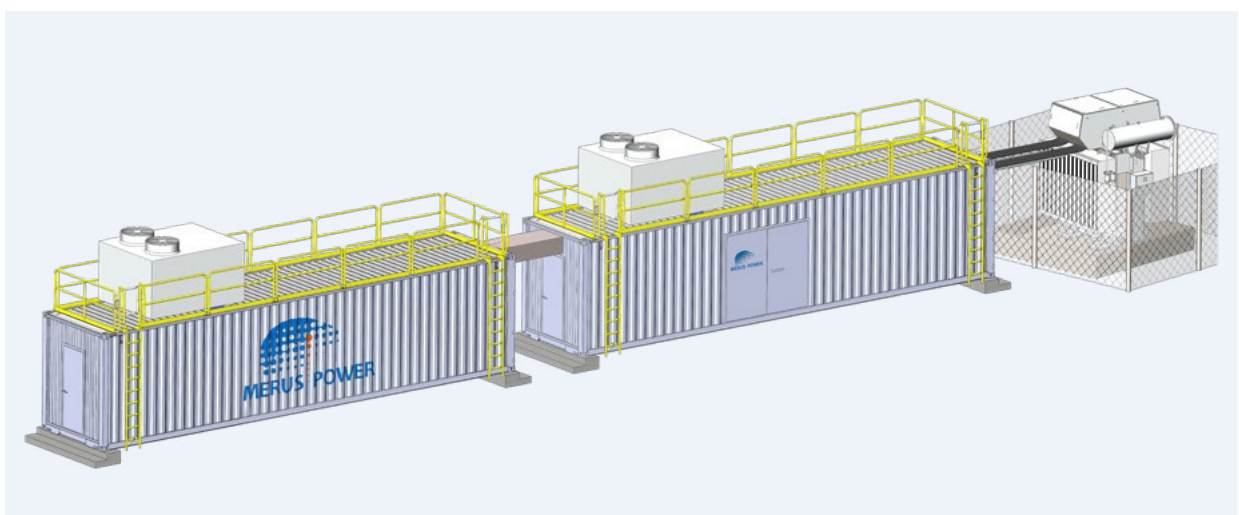
Merus ESS – type 3: Storage and PCS integrated in separate containers. Outdoor power transformer for utility.
